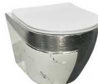
W8043G8 Wall-hung Toilet Size:535x360x360mm P-trap :180mm
